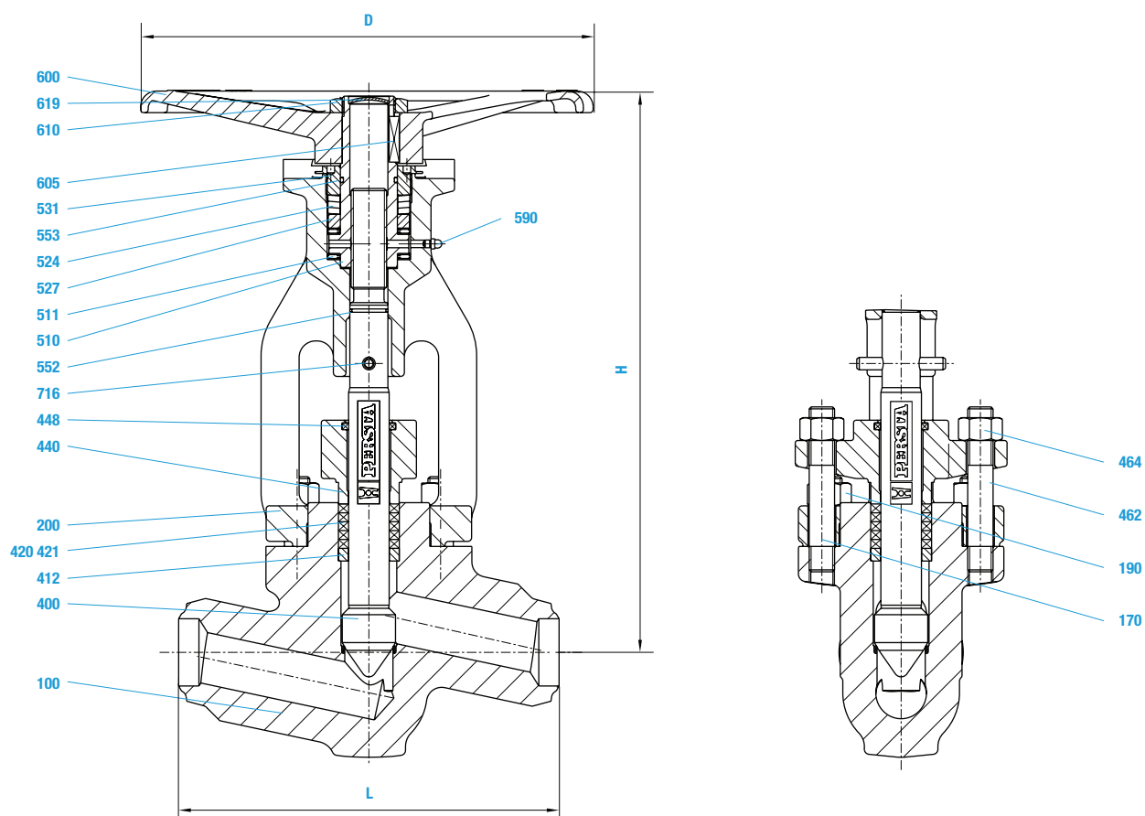
200 LM Shut-off globe valve
